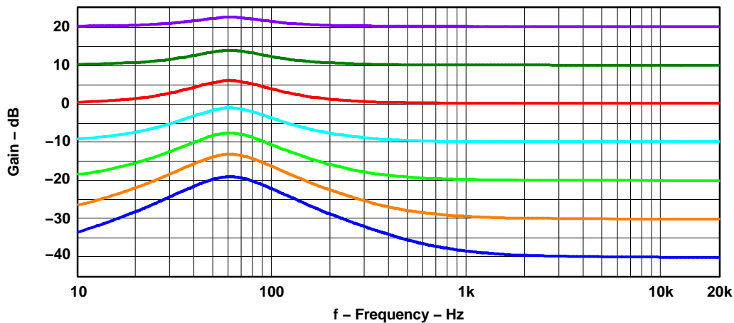
Figure 2-15. Loudness Example Plots
