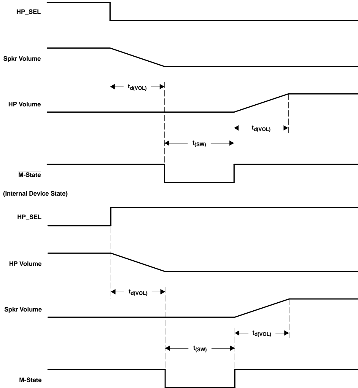
Figure 4-8. \overline{HP\_SEL} Timing
