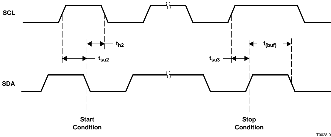
Figure 4-3. Start and Stop Conditions Timing
